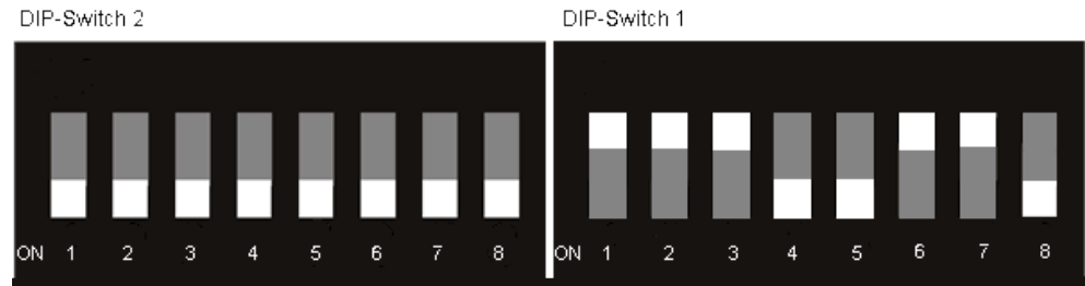
Illustration 12: DIP Switches
